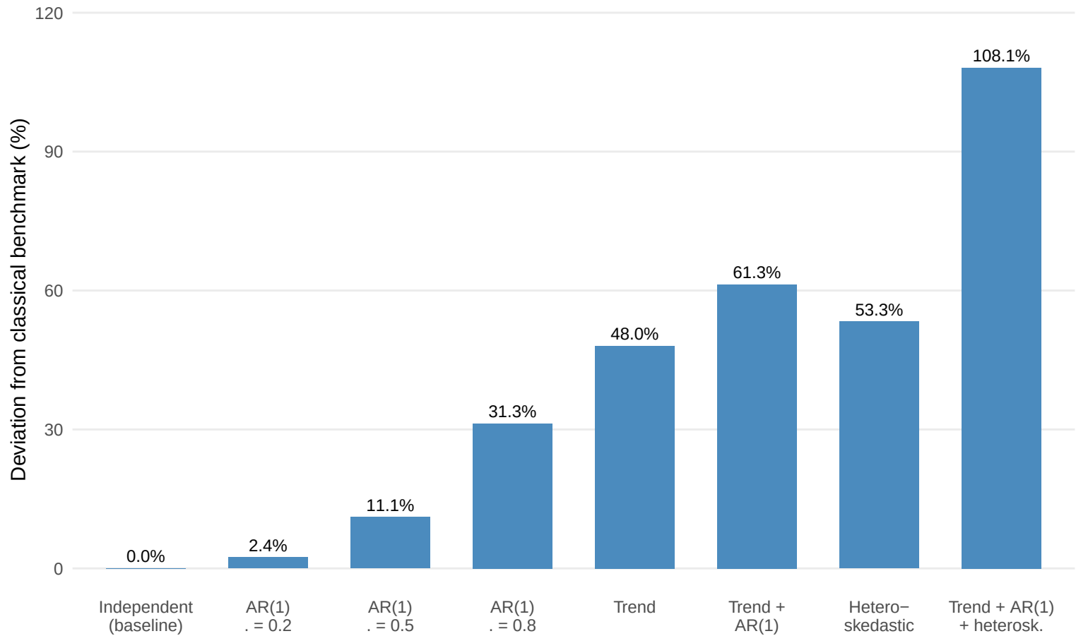
Deviation from classical record-count benchmark across Monte Carlo scenarios
